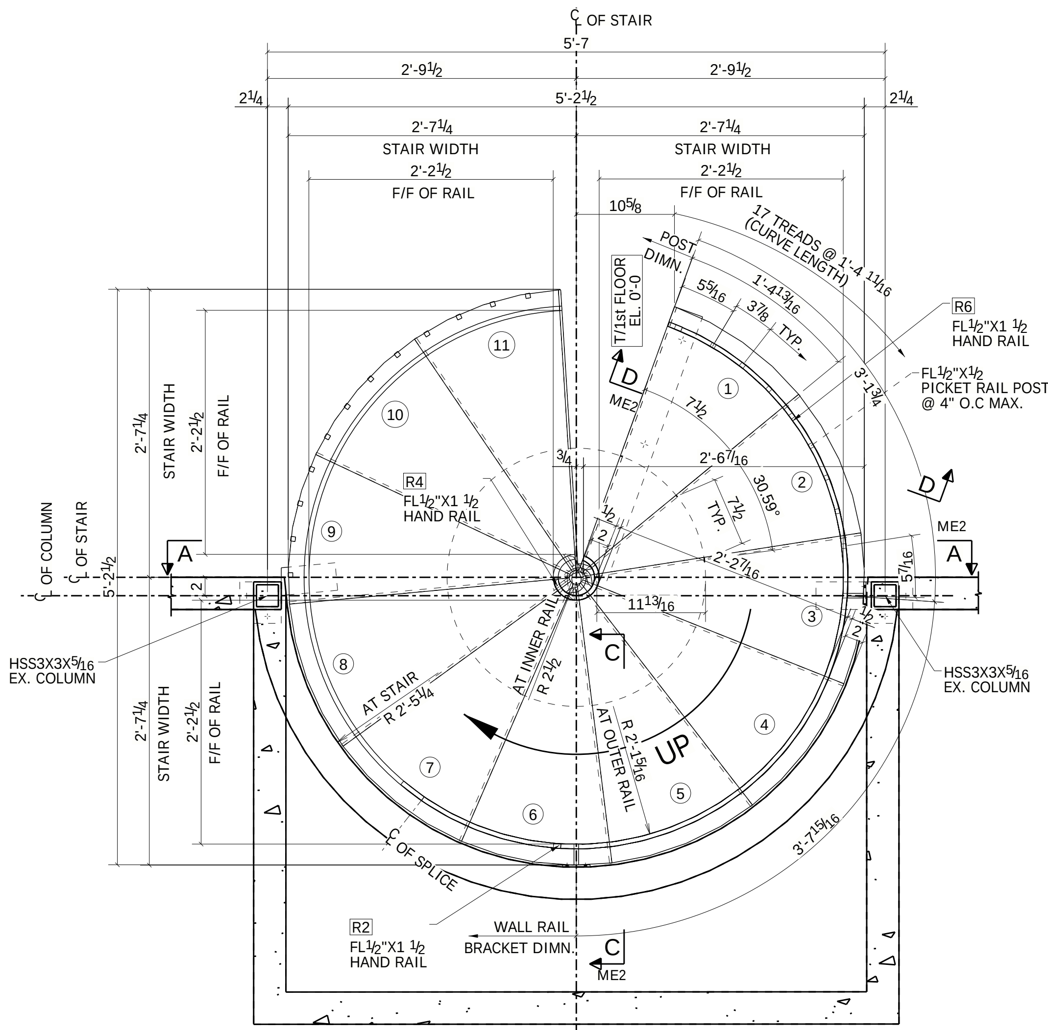
PARTIAL SPIRAL STAIR PH1 FRAMING PLAN AT FIRST FLOOR AT EL. 0 REFER : 1st FLOOR PLAN (1/A2.1)
