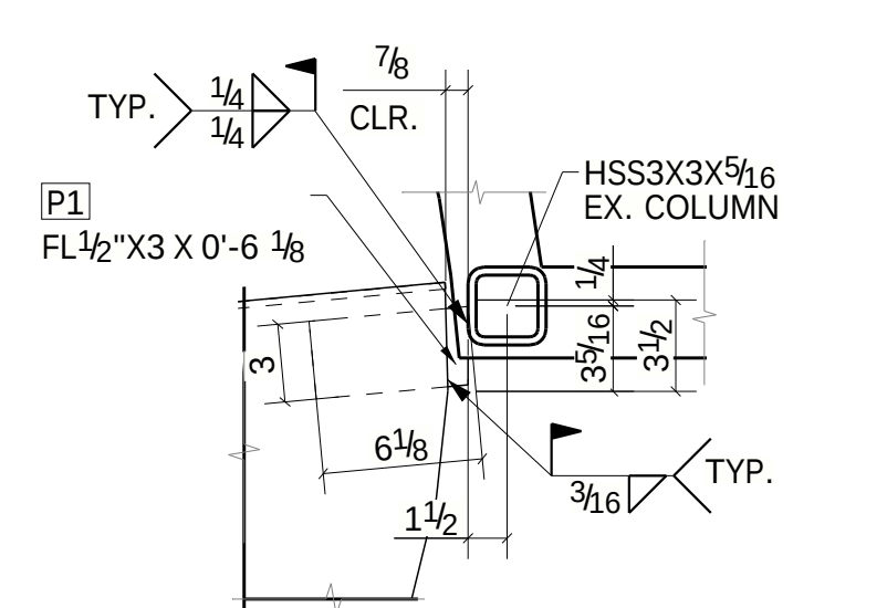
SECTION 4A - 4A
