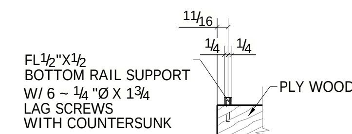
SECTION G1 - G1
