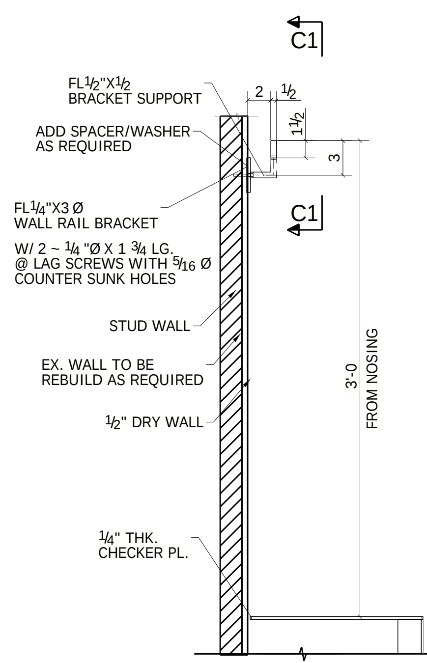
SECTION C - C ME1
