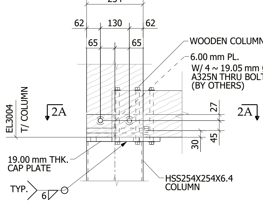
DETAIL-2 ME102
