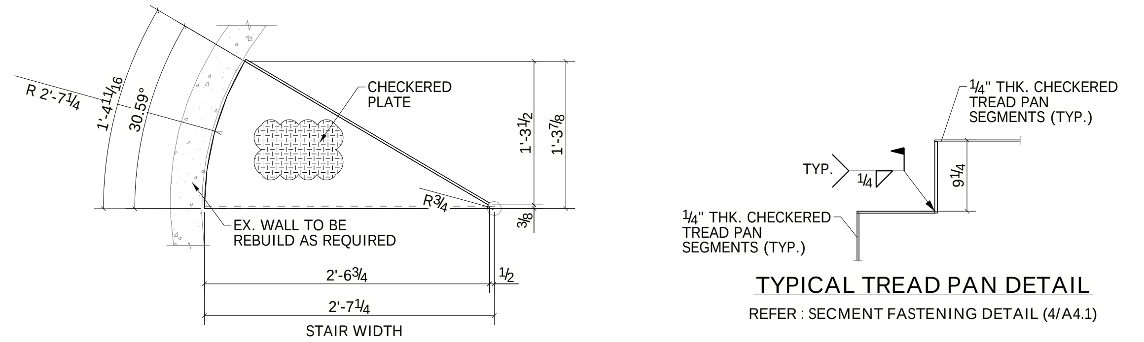
TYPICAL CHECKERED PLATE TREAD PAN DETAIL
