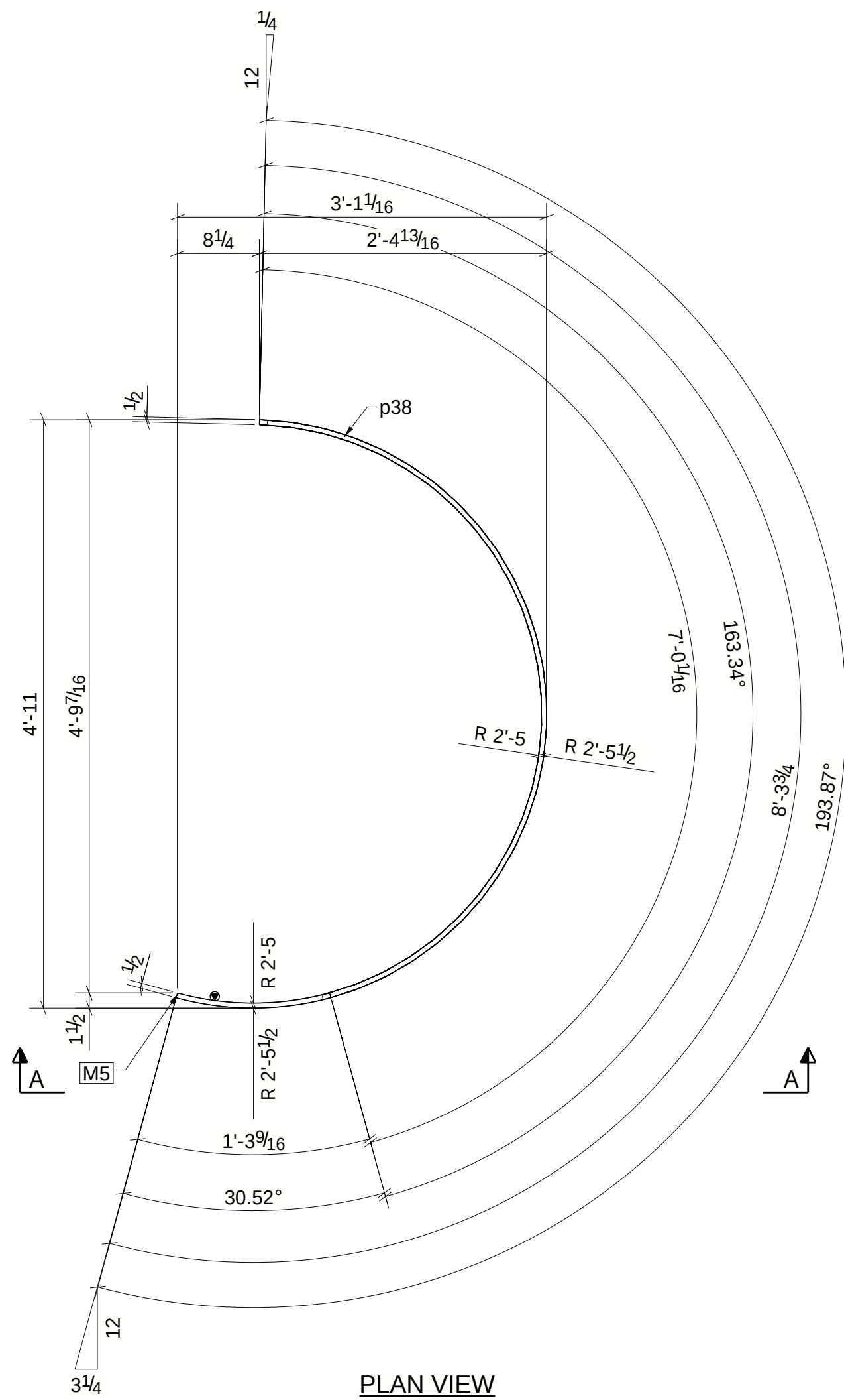
PLAN VIEW
