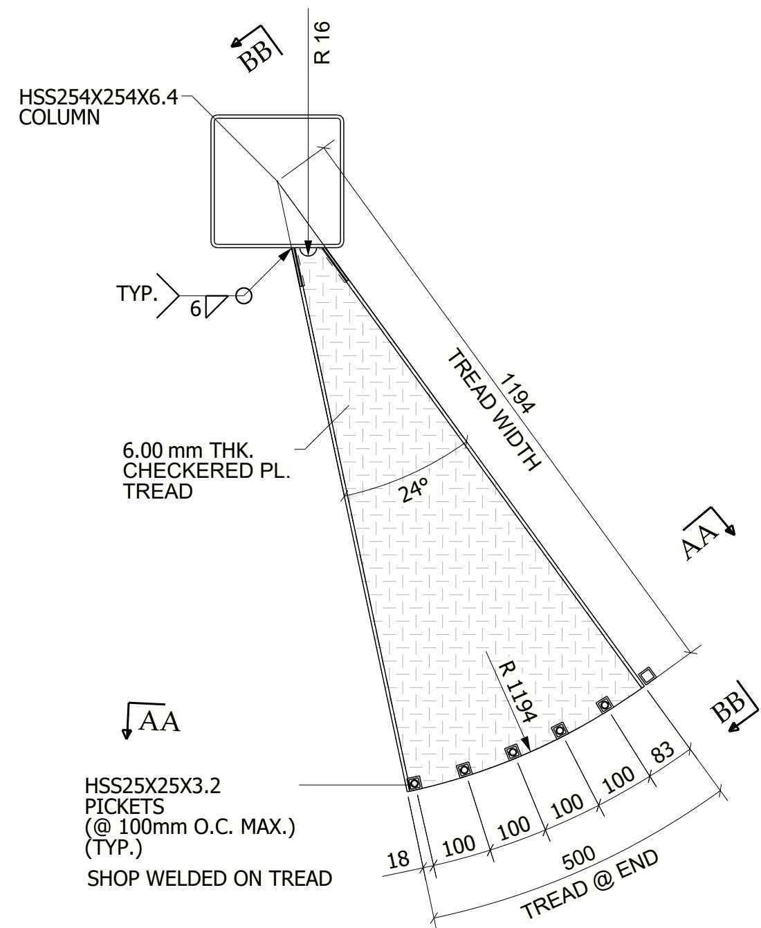
TYPICAL STAIR TREAD DETAIL
