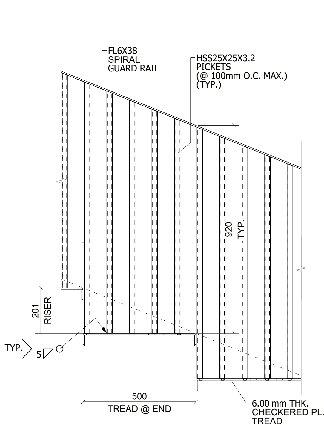
SECTION AA - AA
