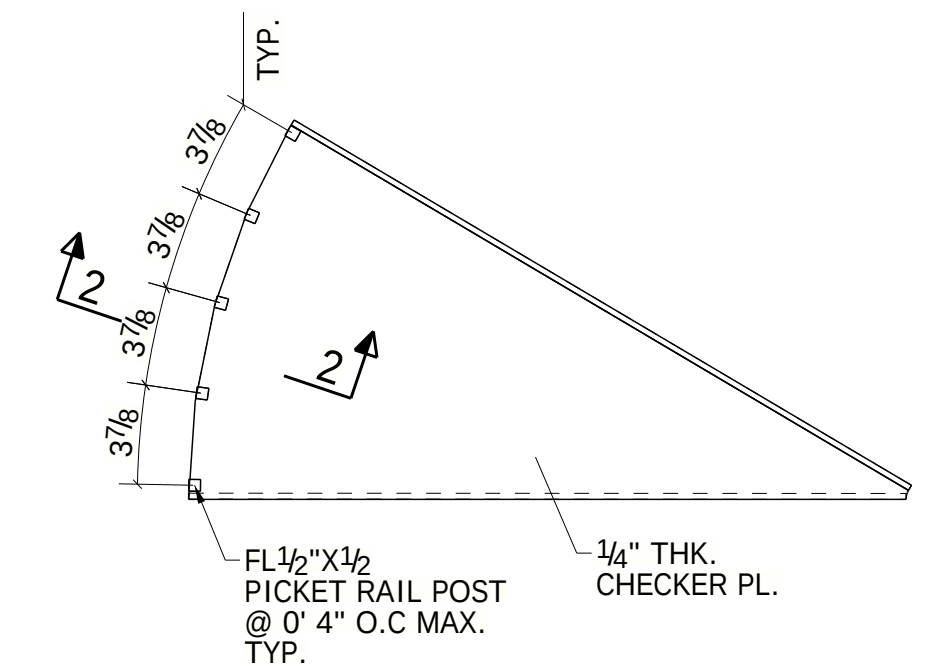
TYPICAL CHECKERED PLATE TO PICKET RAIL POST CONNECTION DETAILS
