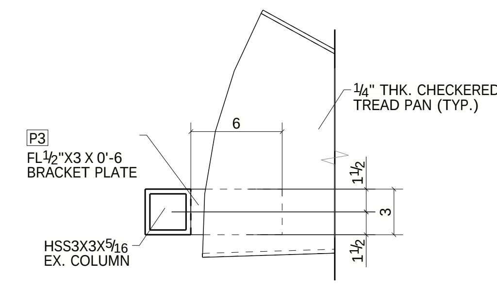
SECTION 5A - 5A
