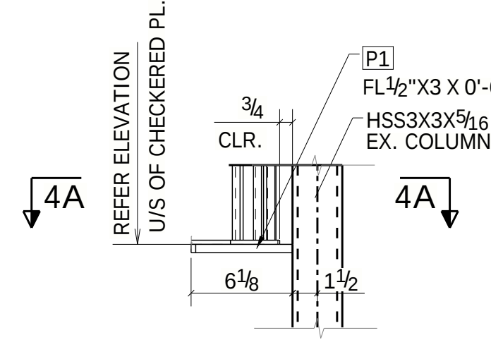
DETAIL 4
