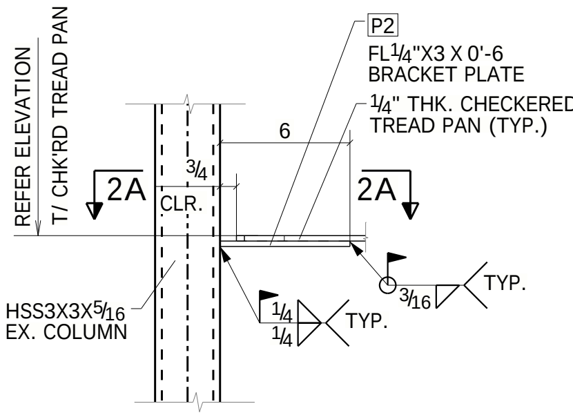
DETAIL 2
