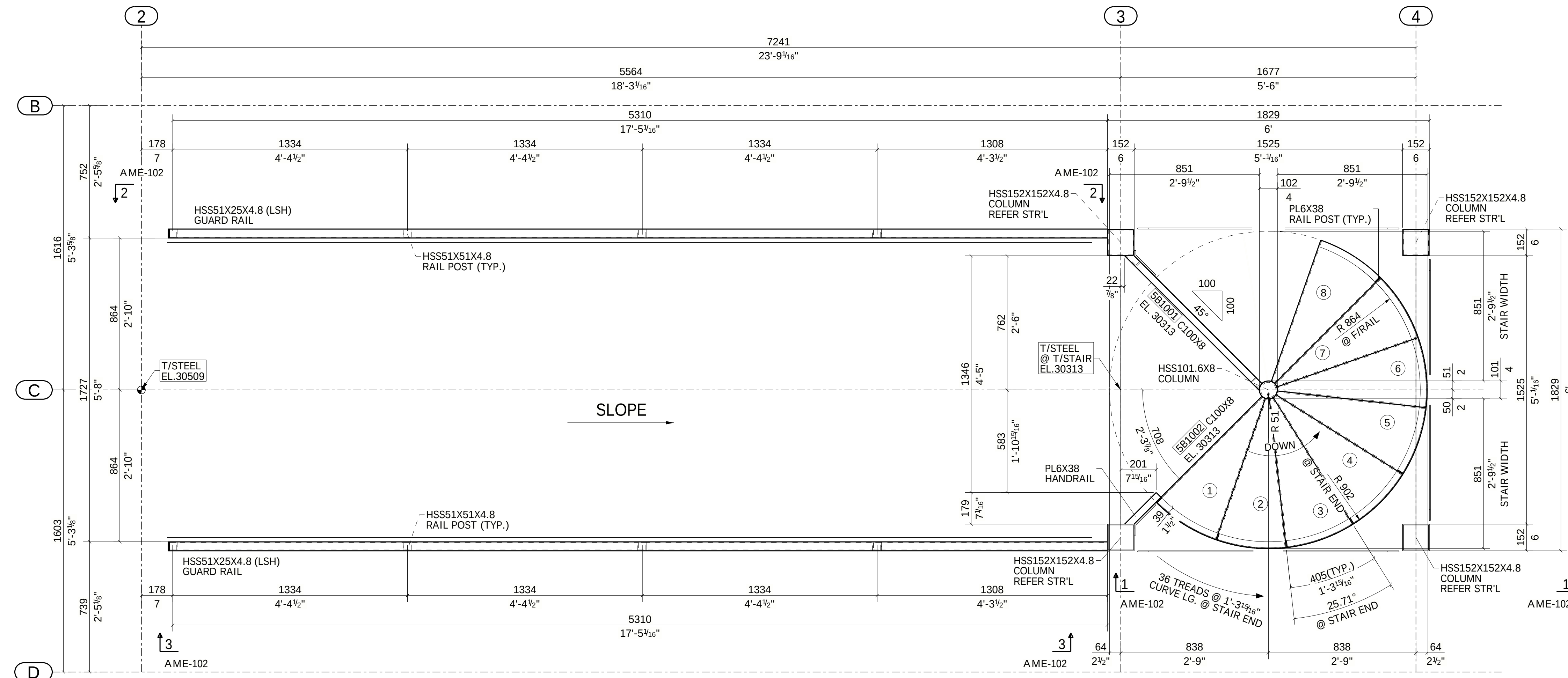
FRAMING PLAN @ WALKWAY - SOUTH CABIN (REFER : PLAN 1:A01/A04)
