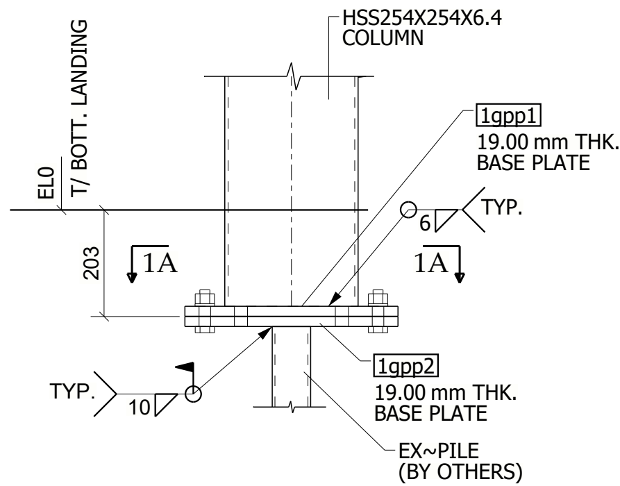
DETAIL-1 ME102
