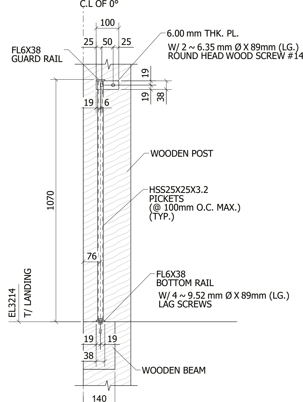
SECTION 2 - 2 ME102
