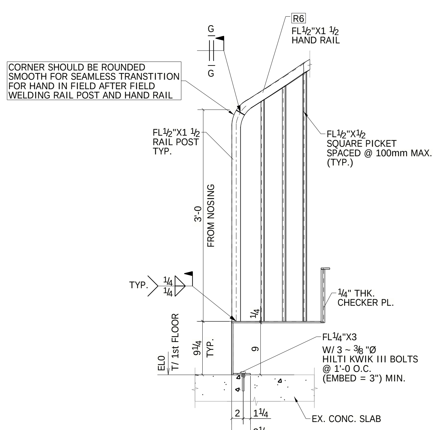
SECTION D - D ME1
