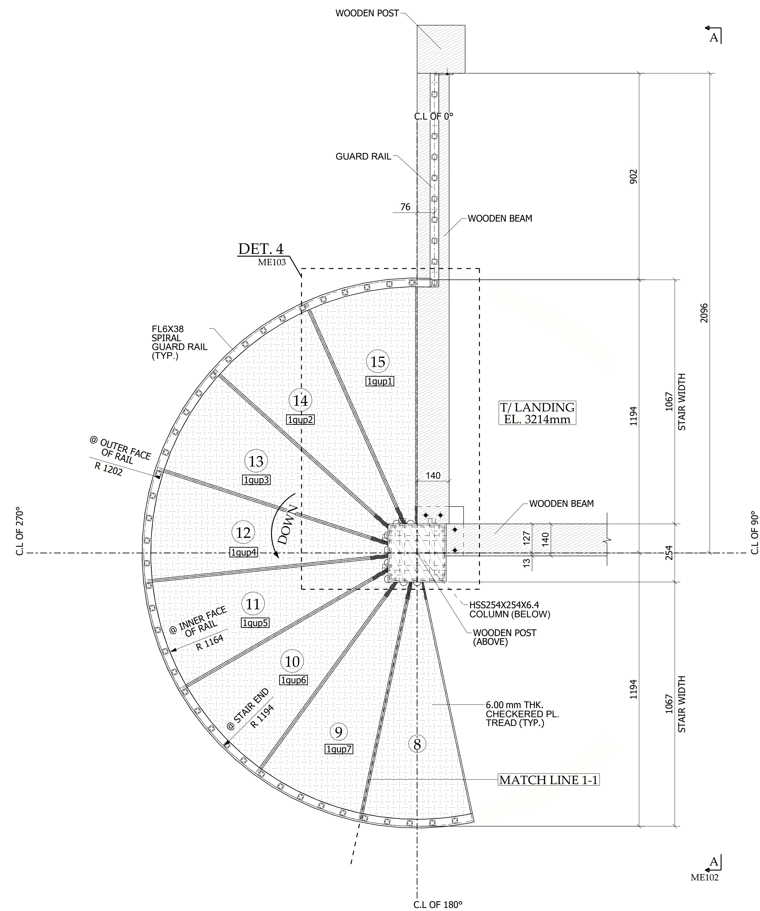
PARTIAL STAIR FRAMING PLAN @ T/LANDING EL. 3214mm
