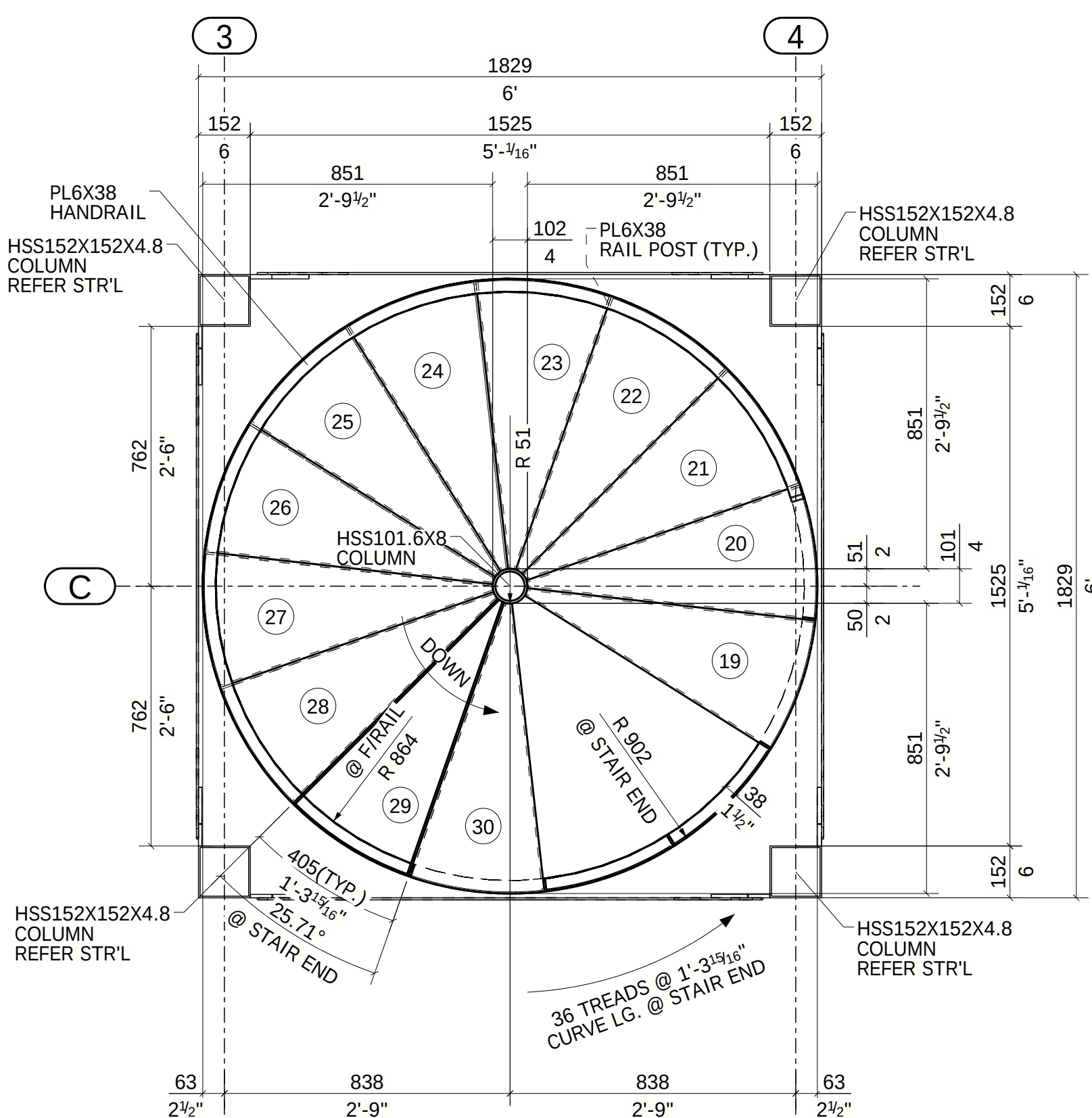
PARTIAL FRAMING PLAN - SOUTH CABIN
