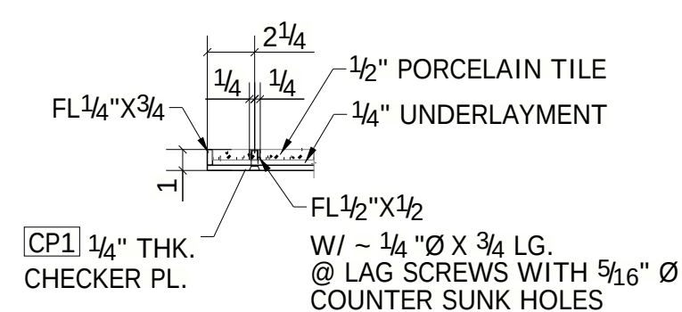
SECTION B1 - B1
