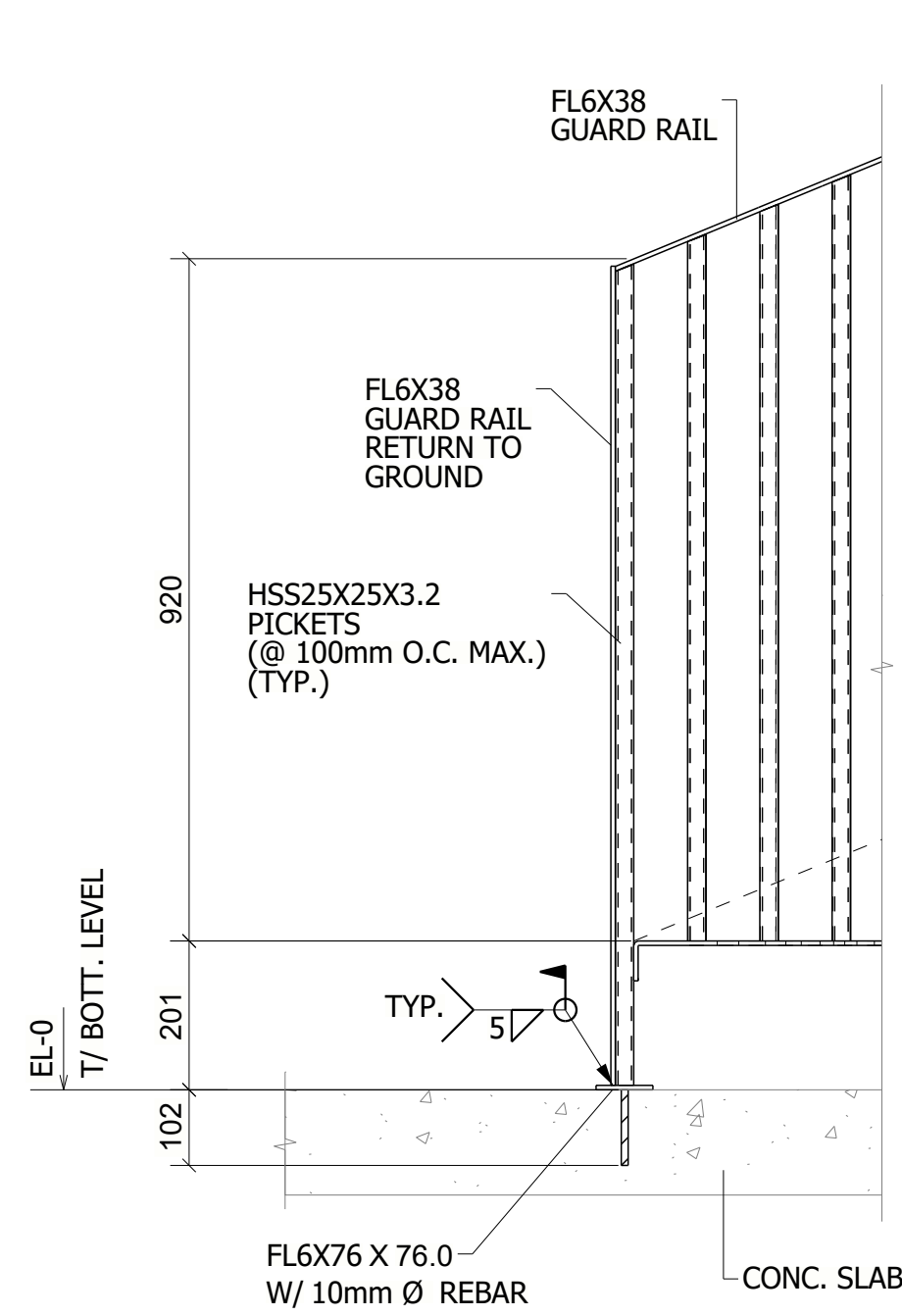
SECTION 1 - 1 ME101
