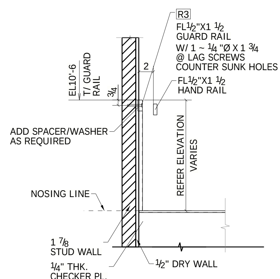
SECTION H - H ME1
