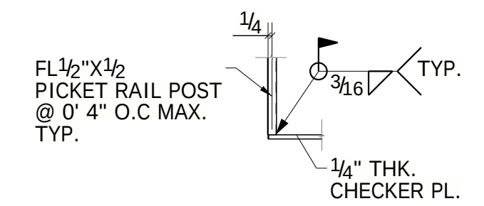
SECTION 2 - 2
