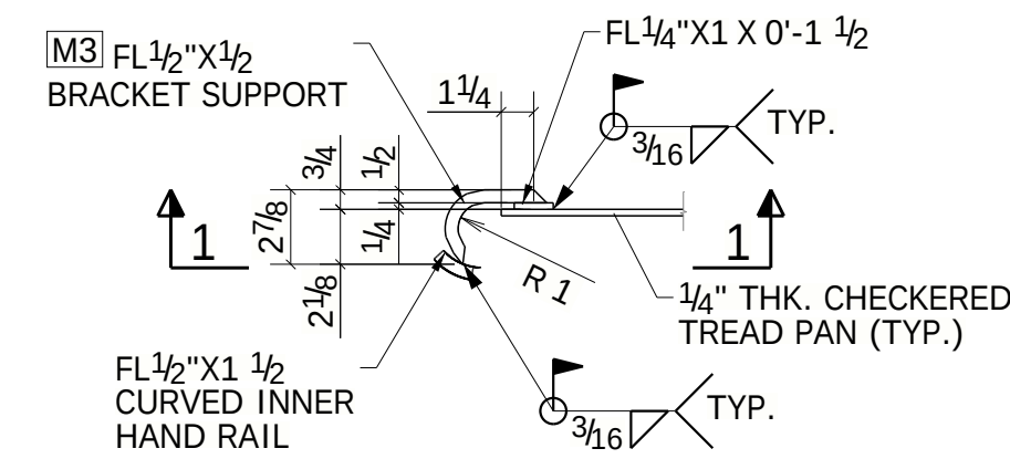
TYPICAL INNER HAND RAIL TO TREAD PAN CONNECTION DETAIL
