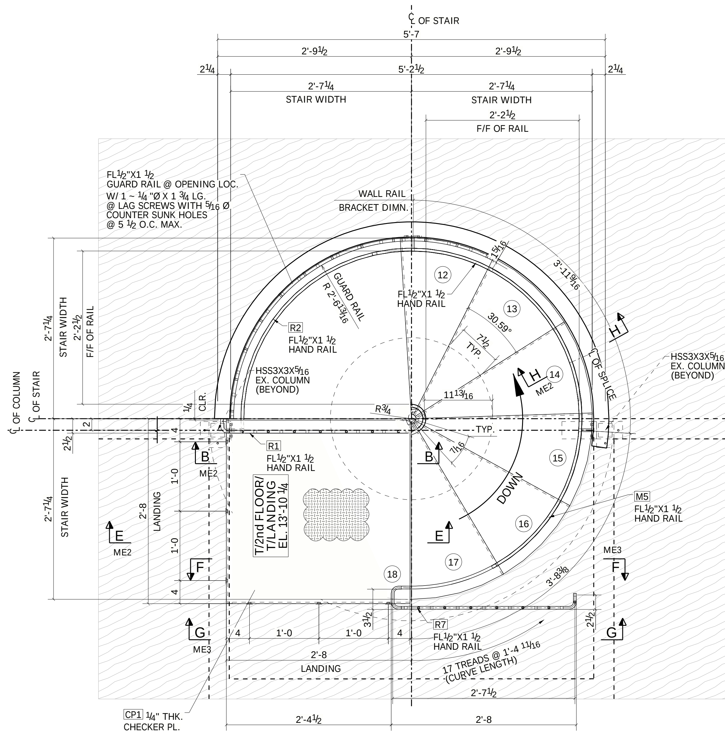
PARTIAL SPIRAL STAIR PH1 FRAMING PLAN AT SECOND FLOOR AT EL. 13'-10 1/4 REFER : 2nd FLOOR PLAN (2/A2.1)
