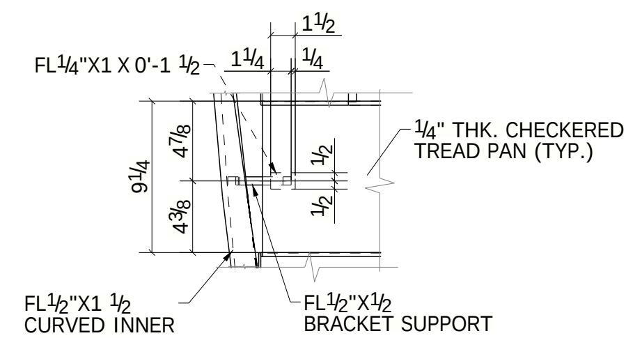
SECTION 1 - 1
