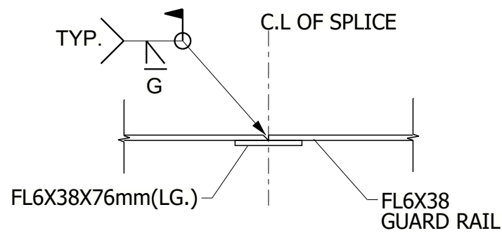
TYPICAL RAIL SPLICE DETAIL
