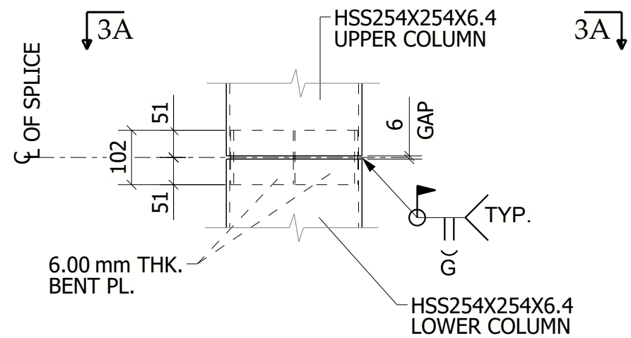
DETAIL-3 ME102
