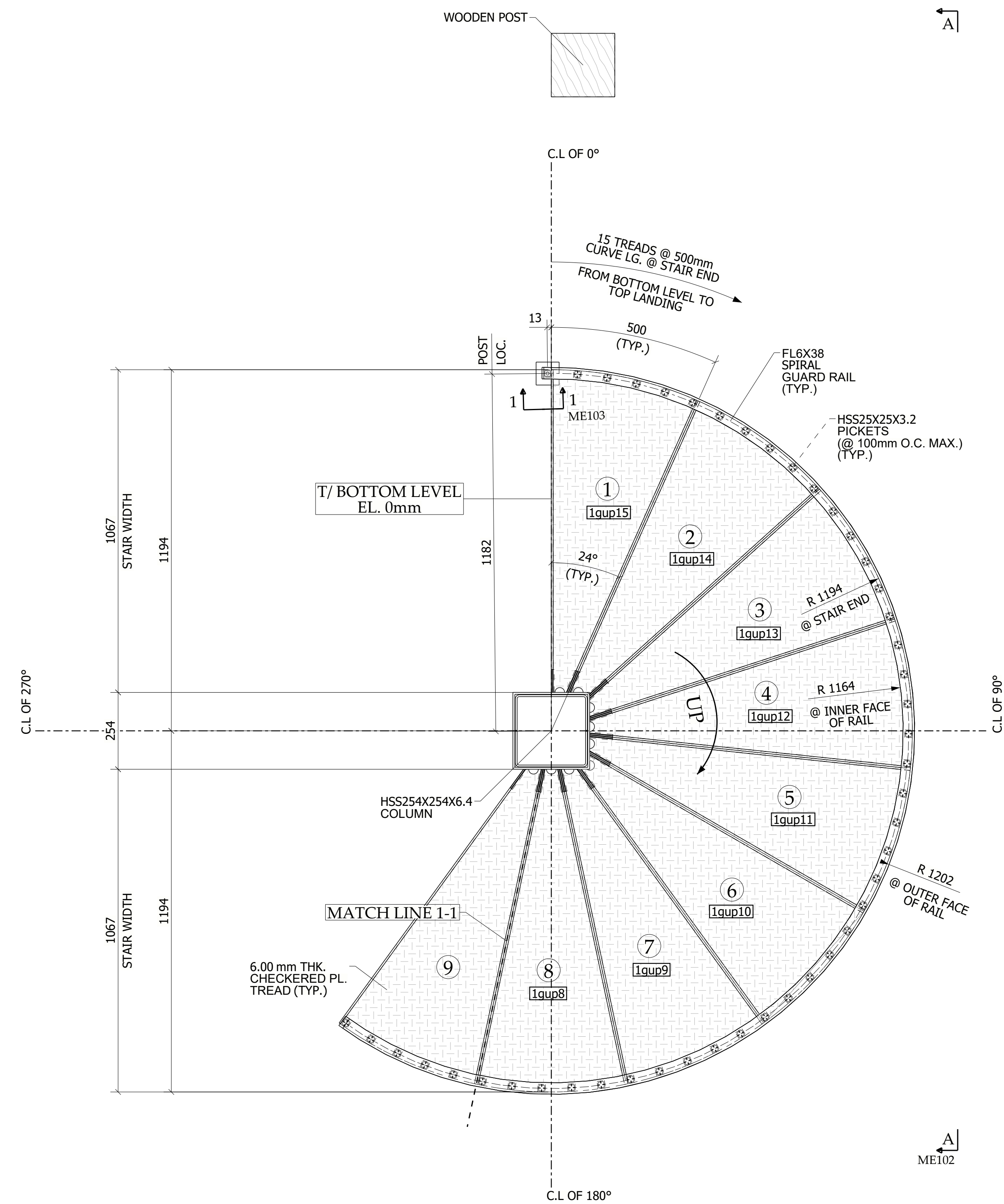
PARTIAL STAIR FRAMING PLAN @ T/BOTTOM LEVEL EL. 0 mm
